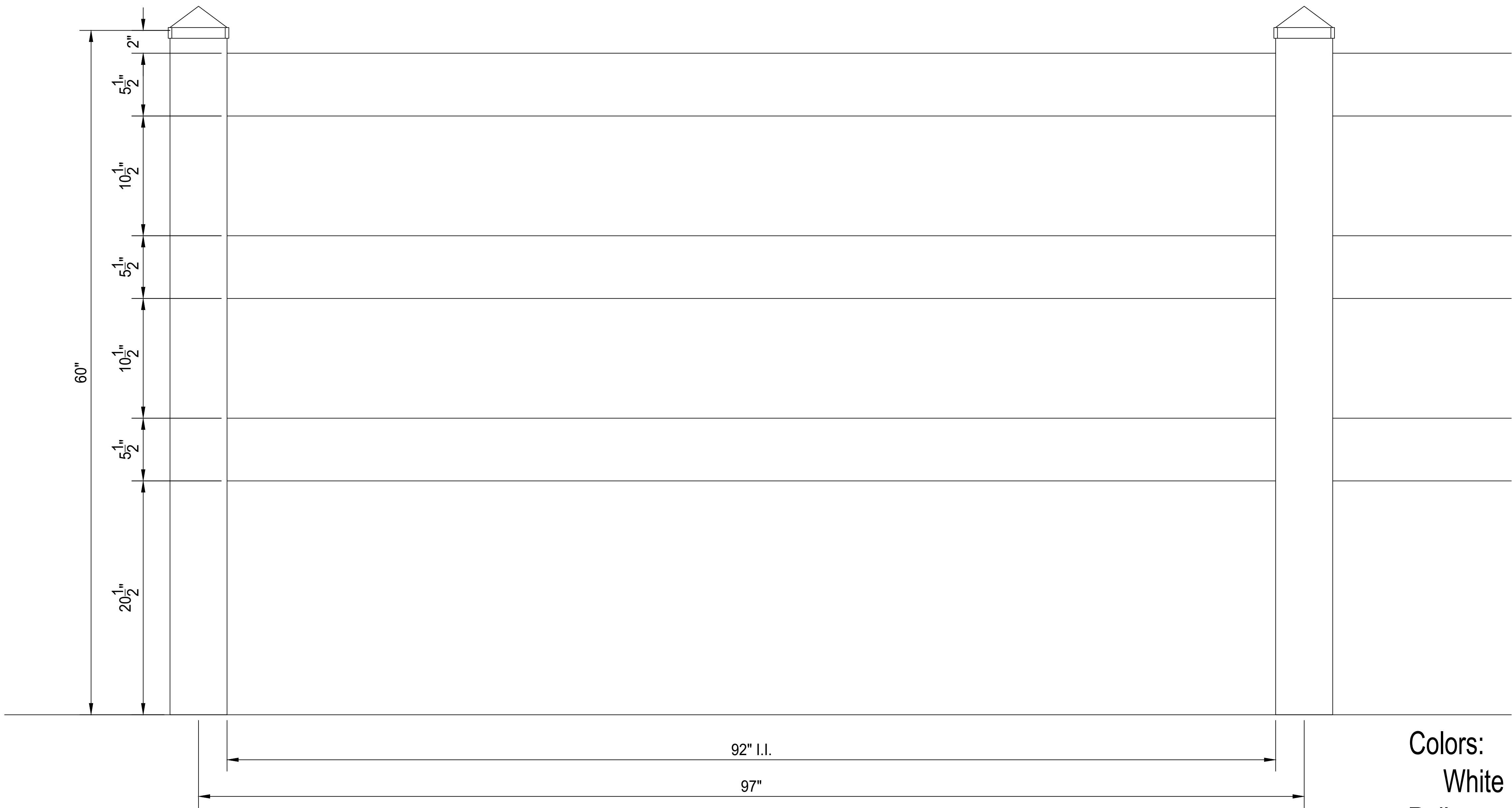
ELEVATION VIEW
